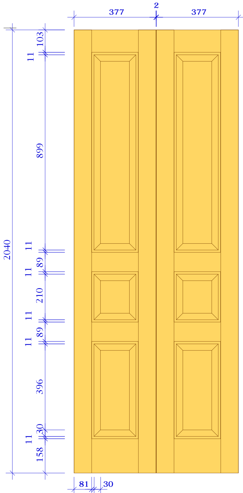
FOLDING DOOR (2M) 1:10
