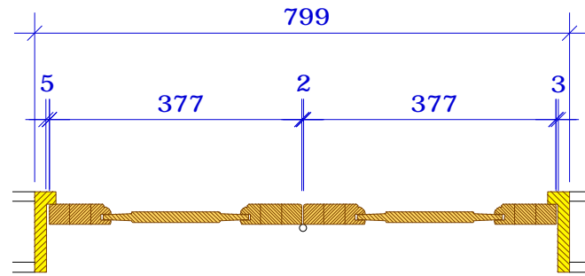
SECTION (2M) 1:10
