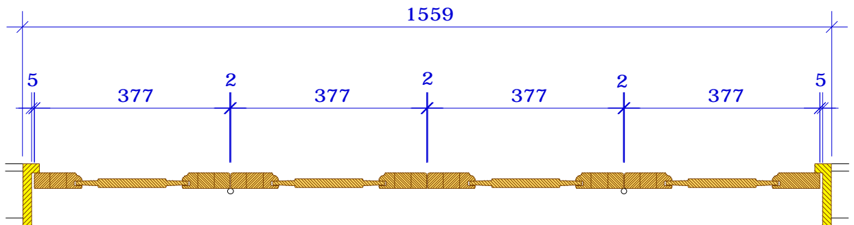
FOLDING DOOR (4M) 1:10
