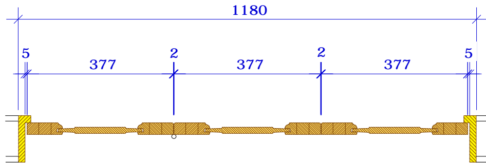
SECTION (3M) 1:10
